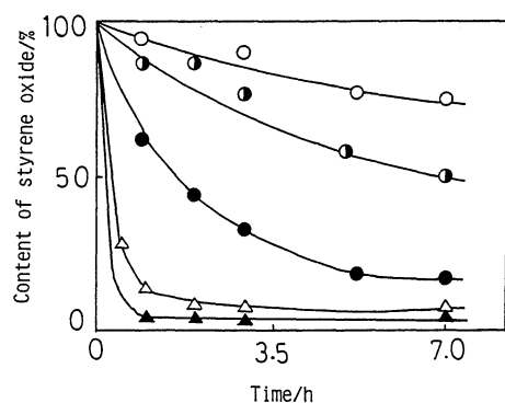
Fig. 2. Effect of \text{Bu}_3\text{N} addition on the activity in the oxidation of styrene: \circ , 0.7 mmol; \bullet , 0.42 mmol; \bullet , 0.35 mmol; \Delta , 0.175 mmol; \blacktriangle , none. 4 (14.6 mmol), \text{H}_2\text{O}_2 (60%, 21.9 mmol), Mob (50 mg), 3 (0.35 mmol), \text{Bu}_3\text{N} , and \text{CHCl}_3 (5 ml) were used. The reaction was carried out at 25 °C.
